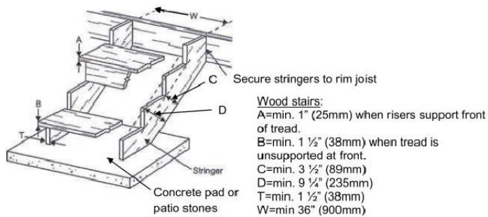
Figure 7 - Stair Detail
