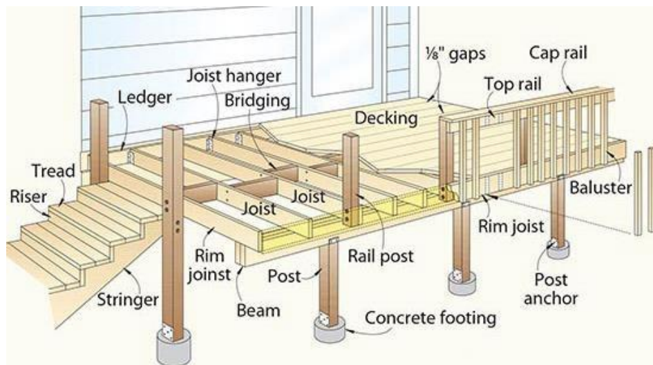
Figure 1a: Deck with labeled components.
