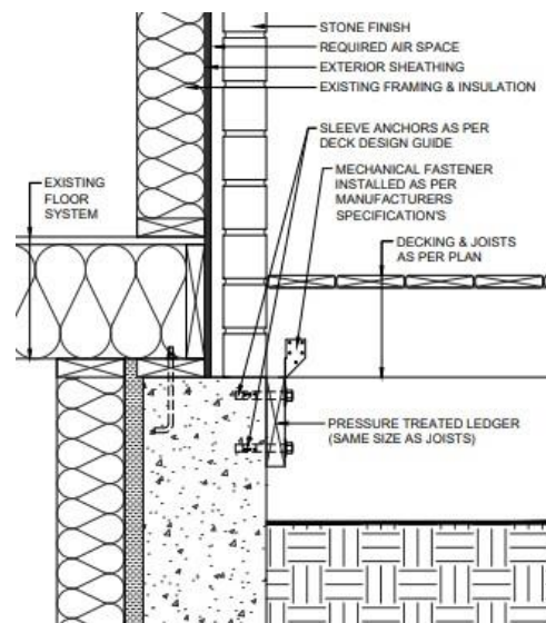
Figure 4b - Deck Connection with Brick
