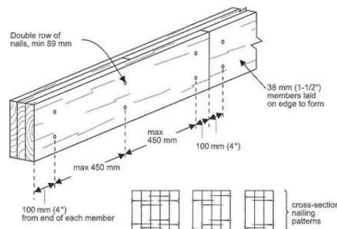
Figure 6 - Built-Up Beam Nailing
