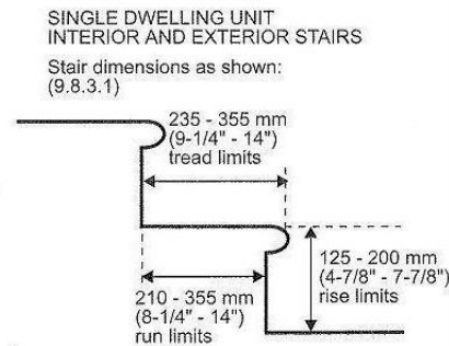
Figure 8 - Stair Dimension
