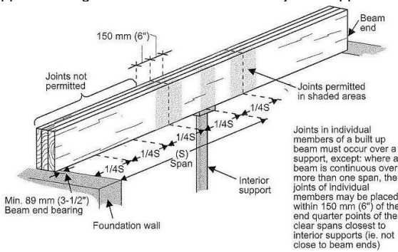
Figure 5a - Built-Up Beam Joints
